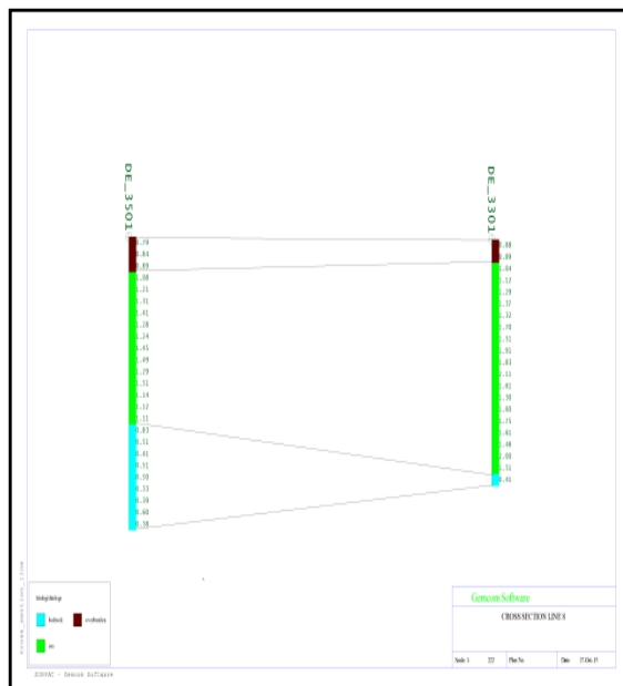
Gambar 9. Cross Section Line 8
