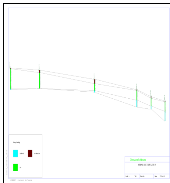
Gambar 6. Cross Section Line 5
