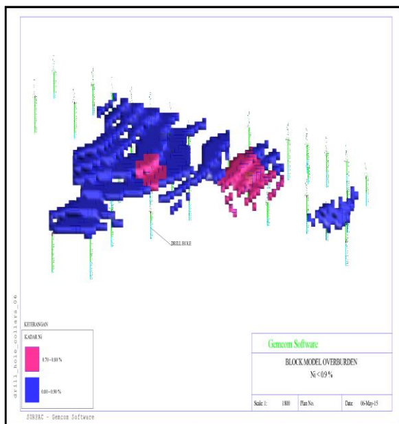
Gambar 10. Block model over burden Ni < 0,9 %
