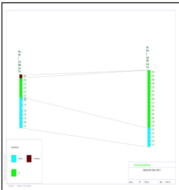
Gambar 8. Cross Section Line 7
