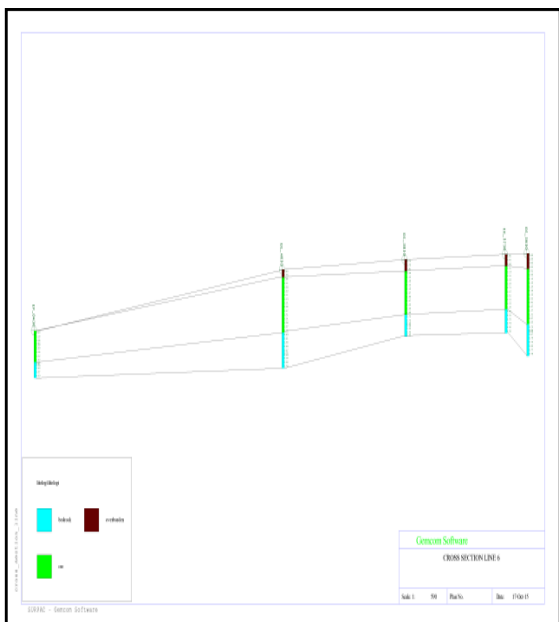
Gambar 7. Cross Section Line 6
