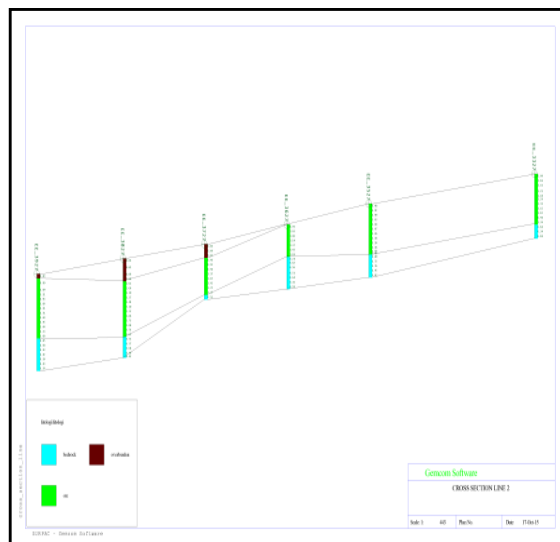
Gambar 3. Cross Section Line 2
