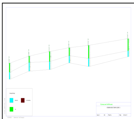
Gambar 2 . Cross Section Line 1
