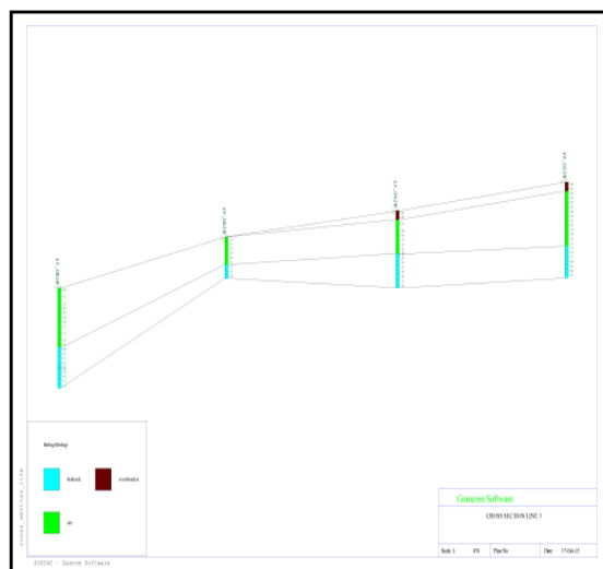
Gambar 4. Cross Section Line 3
